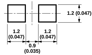
Figure 9. Recommended Soldering Pattern for HSMB-C170.
