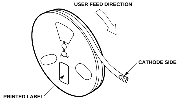
Figure 13. Reeling Orientation.
