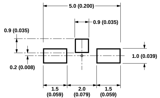
Figure 11. Recommended Soldering Pattern for HSMB-C110.
